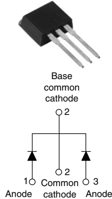
TO-262
